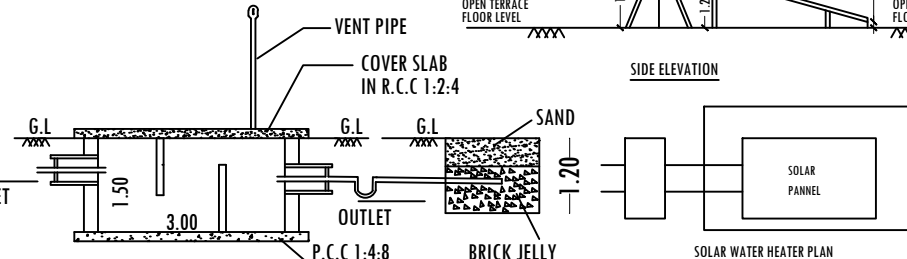
SECTION-AB
