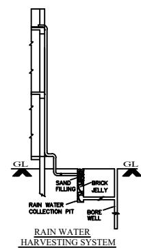
PERCOLATION PIT
