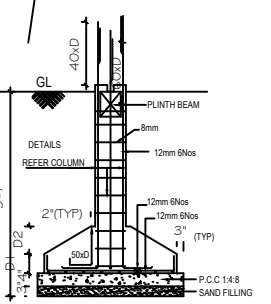
FOUNDATION DETAILS
