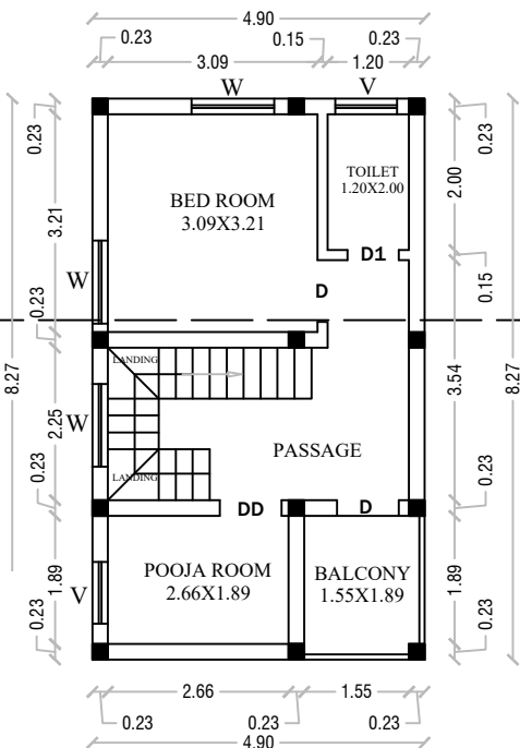
FIRST FLOOR SCALE - 1:100
