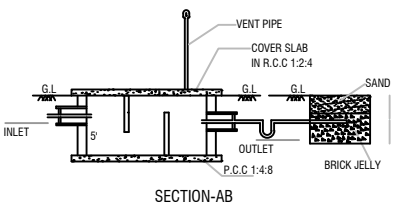
SECTION-AB
