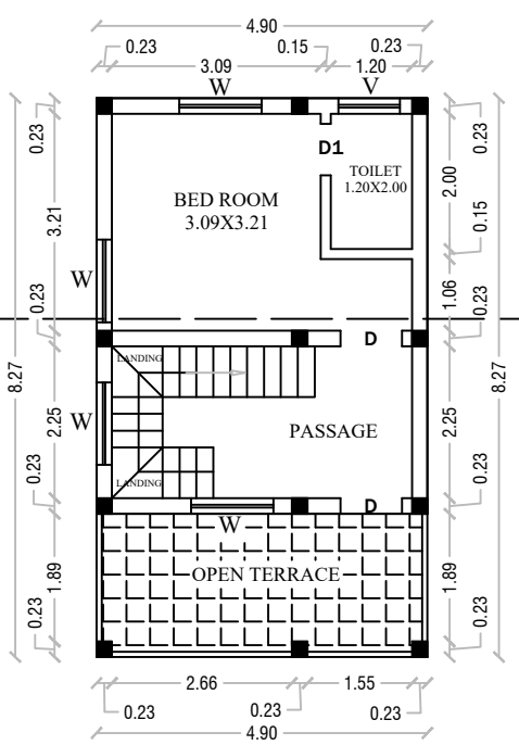
SECOND FLOOR SCALE - 1:100
