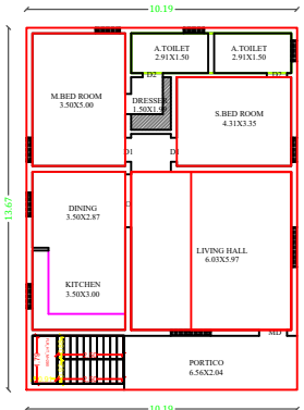
PRO. THIRD FLOOR PLAN.
