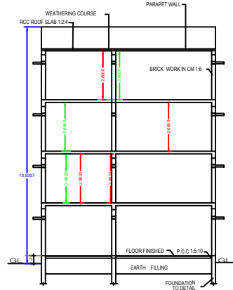
SECTION "A-B"
