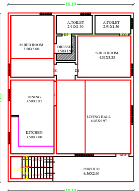
PRO. SECOND FLOOR PLAN.
