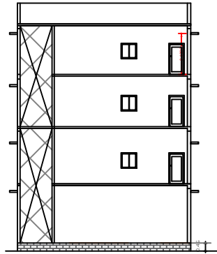
FRONT ELEVATION.
