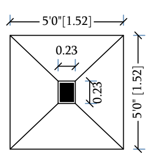
PLAN OF FOUNDATION
