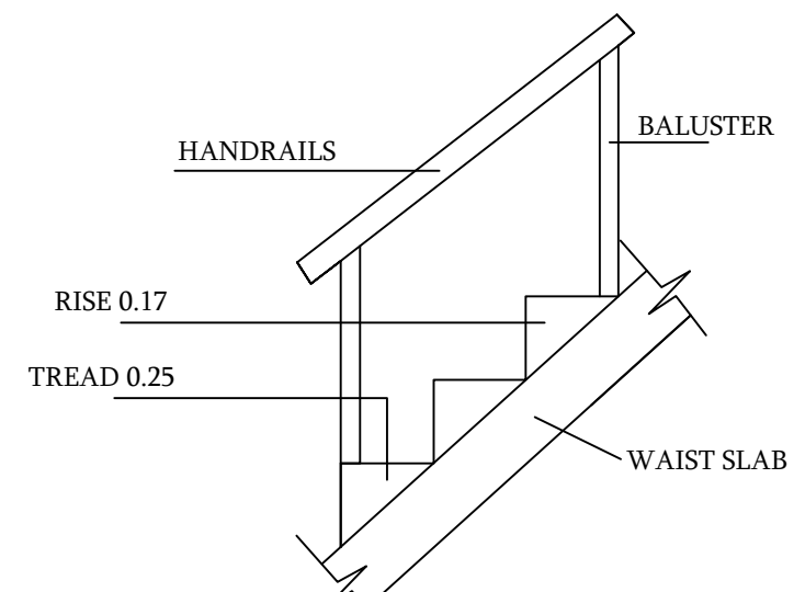
STAIRCASE DETAILS SCALE:1:25
