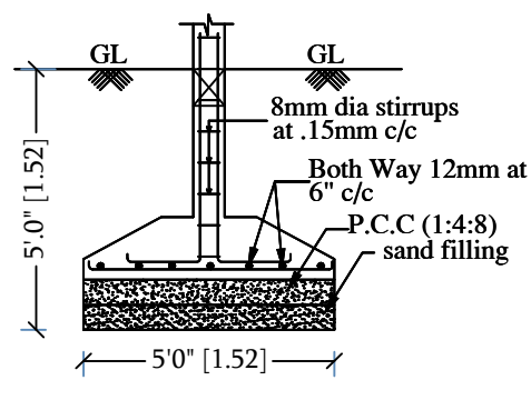
TYPICAL SECTION OF FOOTING
