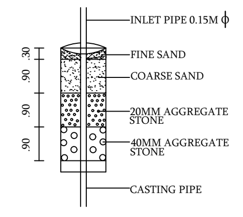
RAIN WATER HAVING SYSTEM
