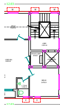
F FLOOR PLAN.
