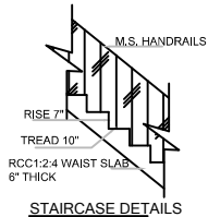
STAIRCASE DETAILS SCALE-1:20
