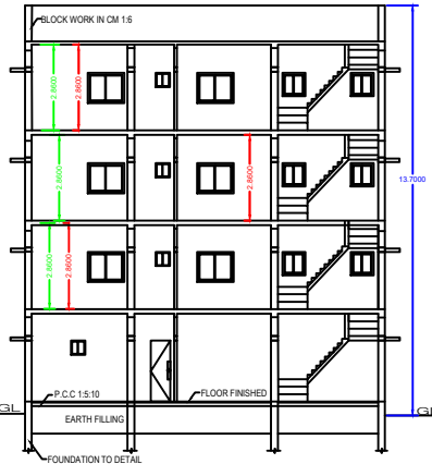
SECTION "A-B"
