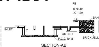
SECTION-A-B
