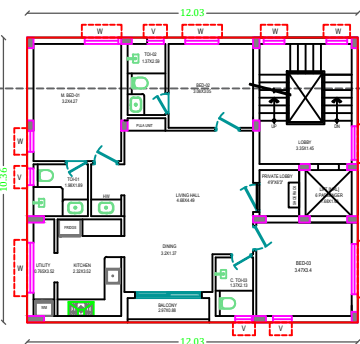
PRO. THIRD FLOOR PLAN.
