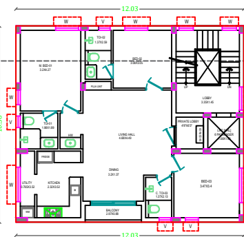
PRO. SECOND FLOOR PLAN.
