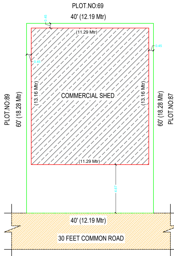
SITE PLAN
