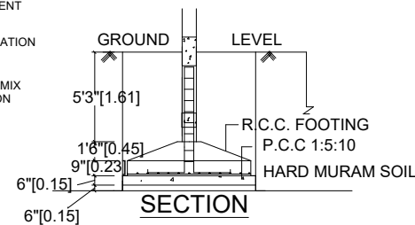
SECTION FOUNDATION DETAILS
