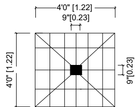
PLAN COLUMN SIZE = 0'9" X 0'9"
