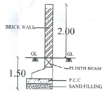
Section
