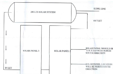
200 LTS SOLAR SYSTEM (TYP) INDIVIDUAL HOUSES SCALE 1:50
