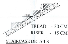
STAIRCASE DETAILS
