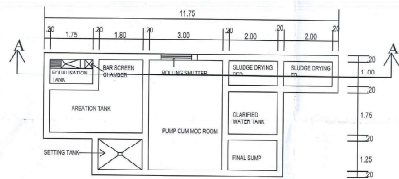
SEWAGE TREATMENT PLANT PLAN
