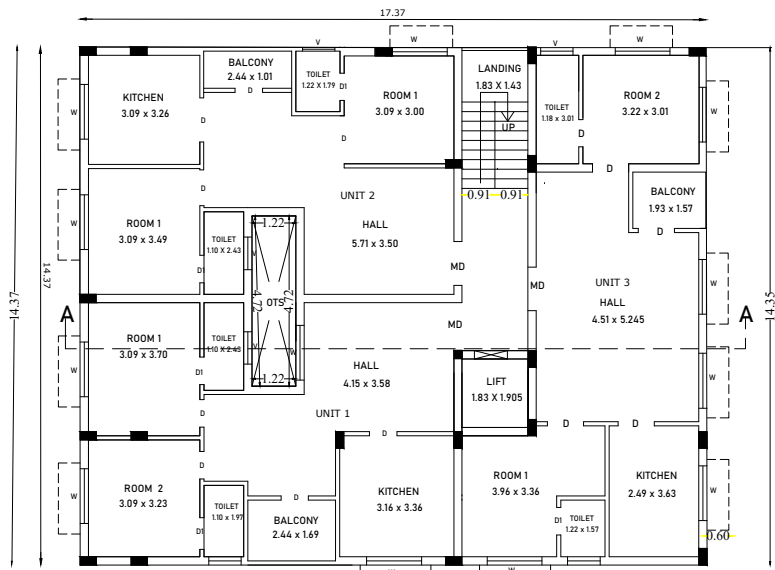
TYPICAL FLOOR PLAN 1ST,2ND,3RD,4TH,5TH
