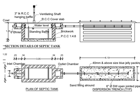
DETAILS OF SEPTIC TANK & DISPERSION TRENCH
