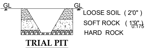
TRIAL PIT
