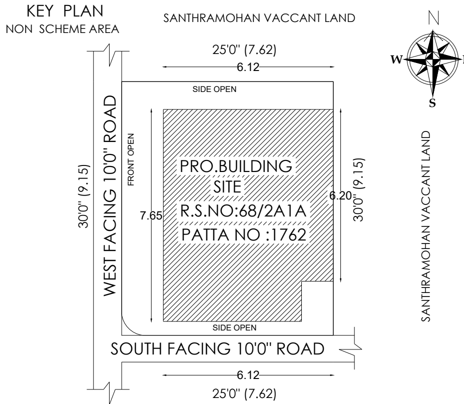
SITE PLAN
