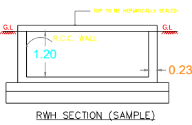
RWH_SECTION (SAMPLE)
