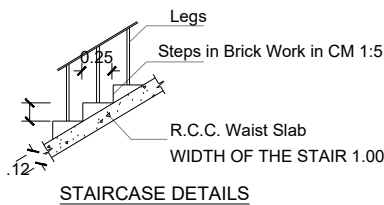
STAIRCASE DETAILS
