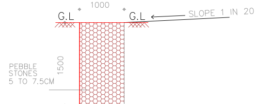
SECTION OF PEBBLE TRENCH
