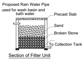
Section of Filter Unit
