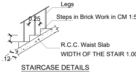
STAIRCASE DETAILS
