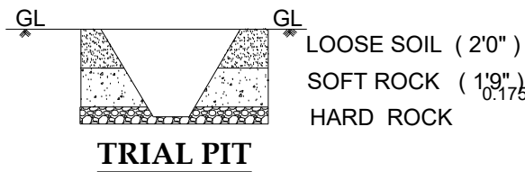
TRIAL PIT
