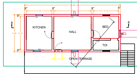
PROPOSED S.F PLAN
