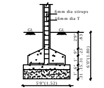
COLUMN FOUNDATION DETAIL
