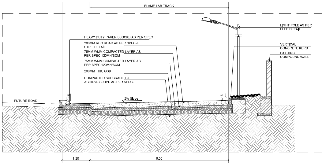
FLAME LAB TRACK SECTION - 1 SCALE : 1: 100
