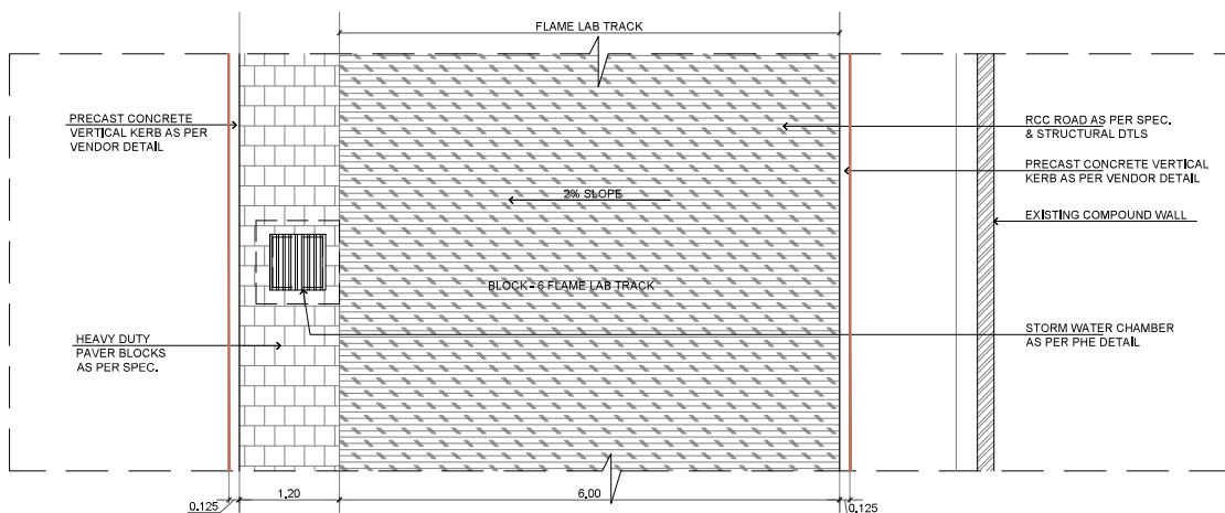
FLAME LAB TRACK PLAN SCALE : 1: 100
