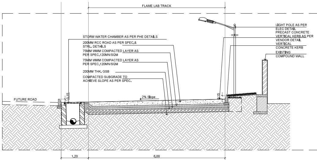
FLAME LAB TRACK SECTION - 2 SCALE : 1: 100
