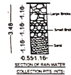
SECTION OF RAIN WATER COLLECTION R.T.S. (R.T.S.)
