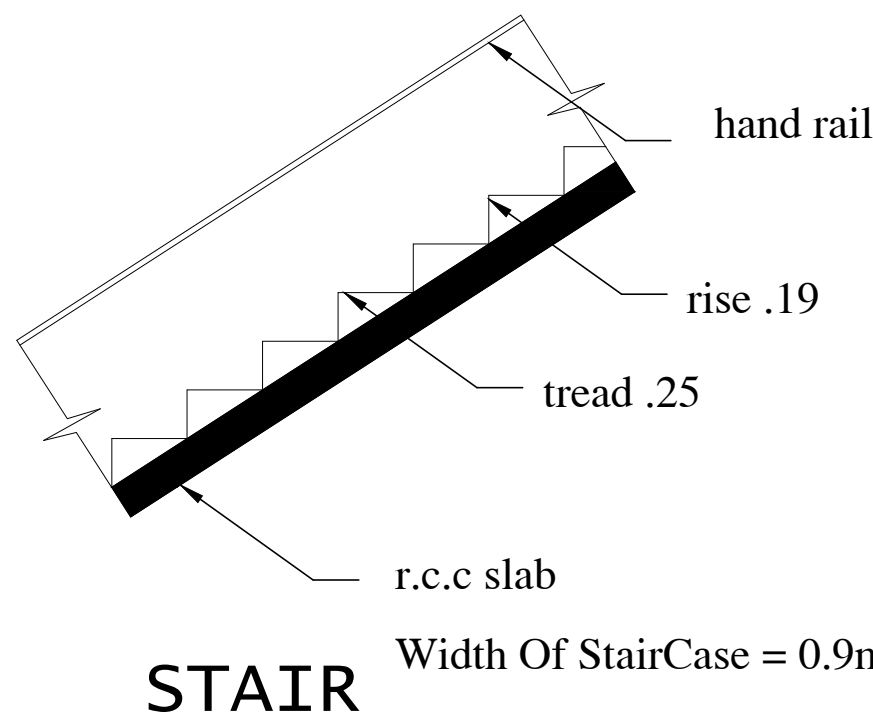
STAIR
