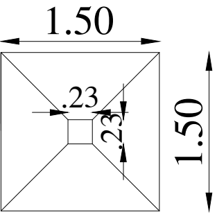
COLUMN FOUNDATION
