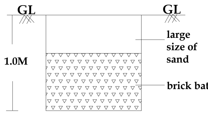
RAINWATER HARVESTING
