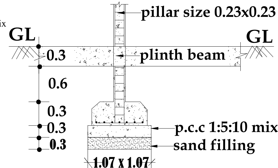
FOUNDATION DETAILS
