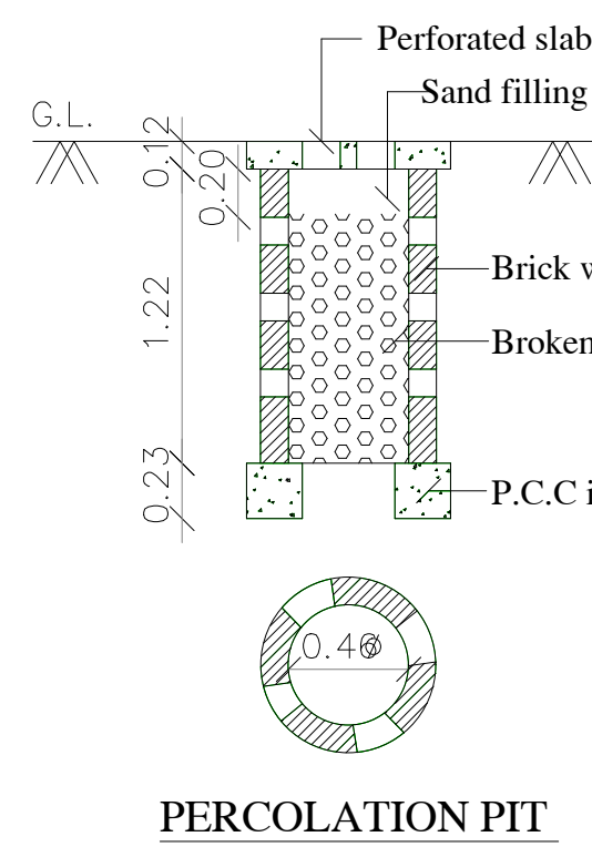
PERCOLATION PIT
