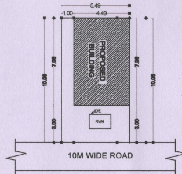
SITE PLAN
