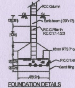
FOUNDATION DETAILS
