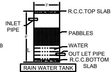
RAIN WATER TANK
