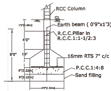
FOUNDATION DETAILS
