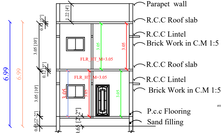
SECTION ON"AA"
