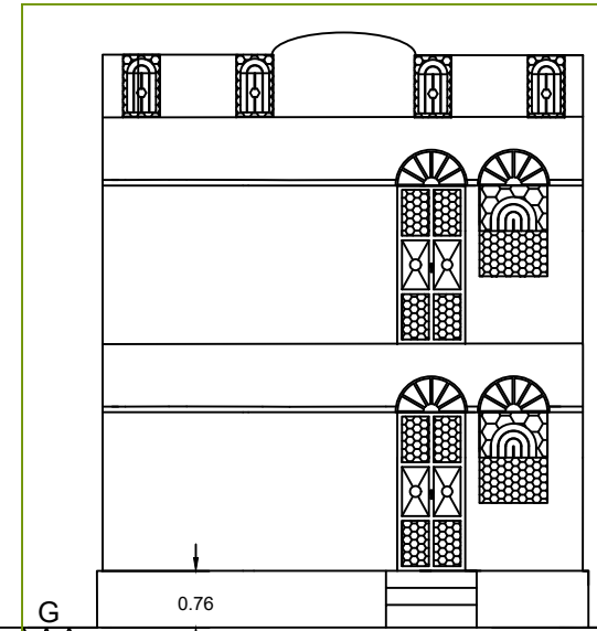
ELIVATION
