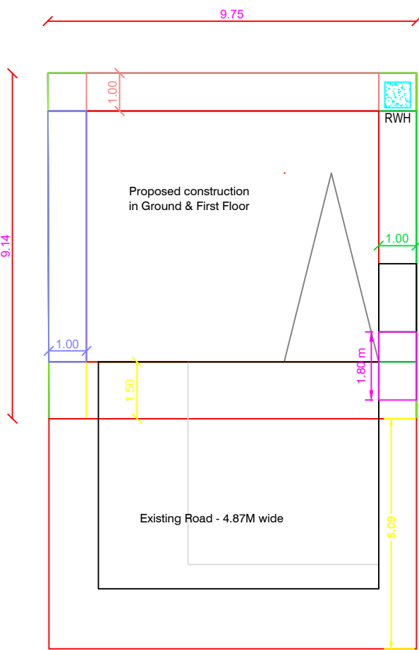
SITE PLAN
