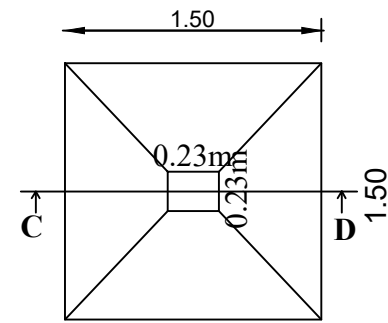
SECTION - 'CD'
