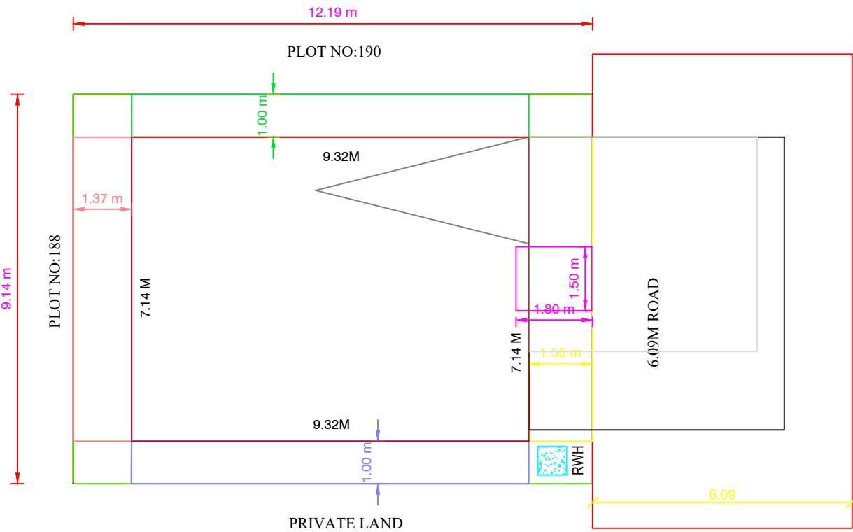
SITE PLAN
