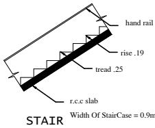
STAIR
