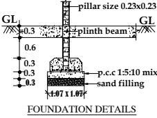
FOUNDATION DETAILS
