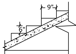
Staircase Detail Not To Scale
