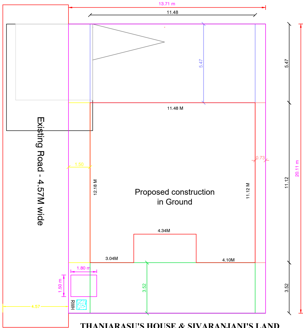
SITE PLAN
