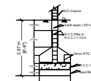
FOUNDATION DETAILS
