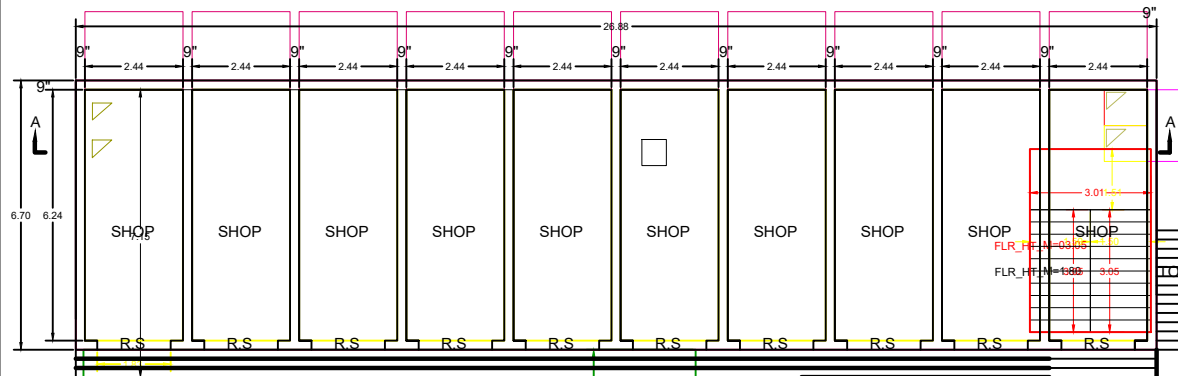
G.F. PLAN
