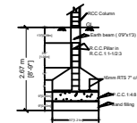
FOUNDATION DETAILS
