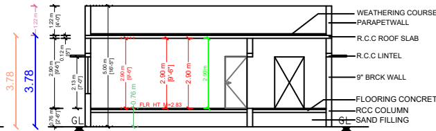
SECTION ON 'A-A'
