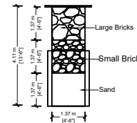
SECTION OF RAIN WATER COLLECTION PITS (NTS)
