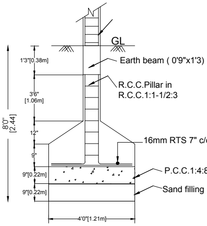
FOUNDATION DETAILS
