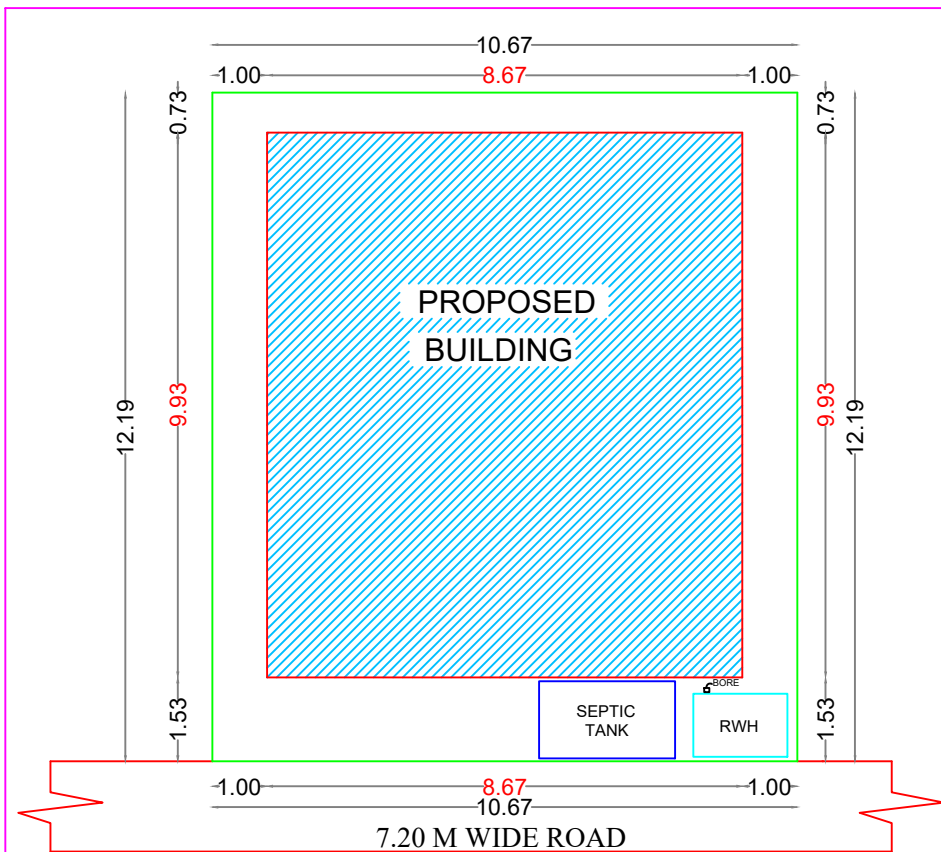
SITE PLAN
