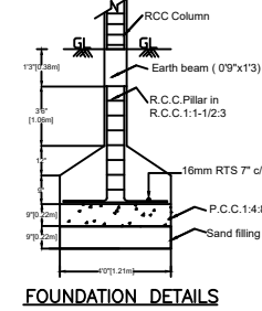
FOUNDATION DETAILS
