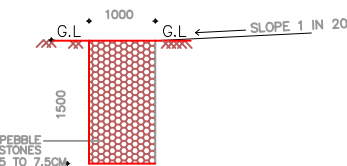
SECTION OF PEBBLE TRENCH SCALE : 1: = 100
