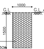
SECTION OF PEBBLE TRENCH SCALE : 1: = 100
