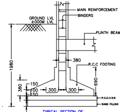
TYPICAL SECTION OF R.C.C. COLUMN FOUNDATION SCALE : 1" = 2'-0"
