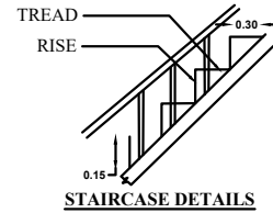
STAIRCASE DETAILS
