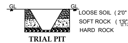
TRIAL PIT
