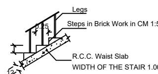
STAIRCASE DETAILS
