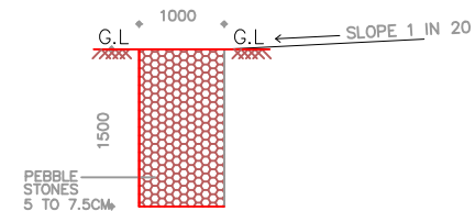
SECTION OF PEBBLE TRENCH SCALE : 1: = 100
