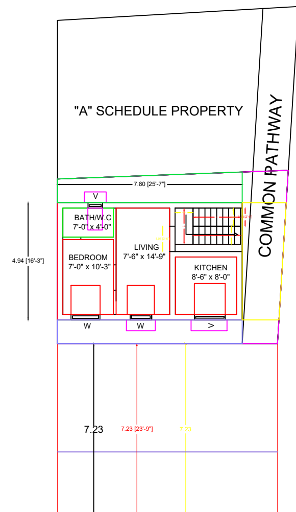
RWH_CAPACITY_L = 2000LTRS
