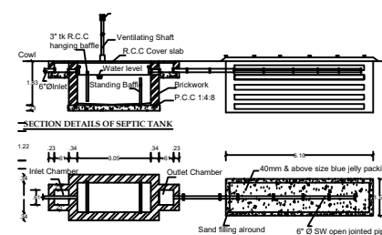
DETAILS OF SEPTIC TANK & DISPERSION TRENCH
