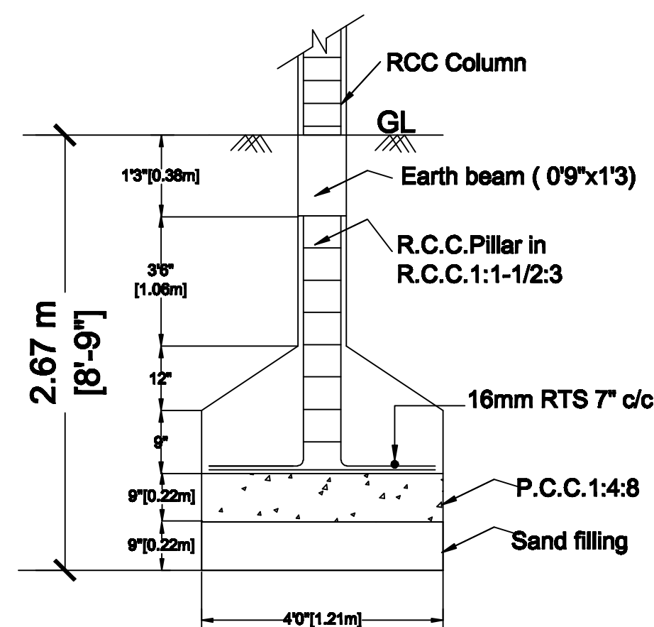
FOUNDATION DETAILS
