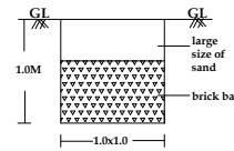
RAINWATER HARVESTING
