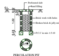
PERCOLATION PIT
