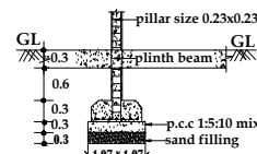
FOUNDATION DETAILS
