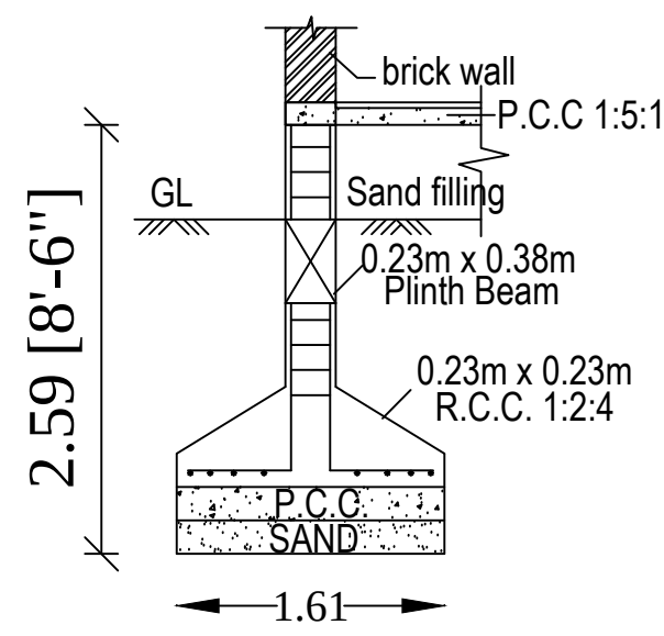
FOUNDATION DETAILS
