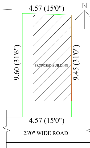
SITE PLAN
