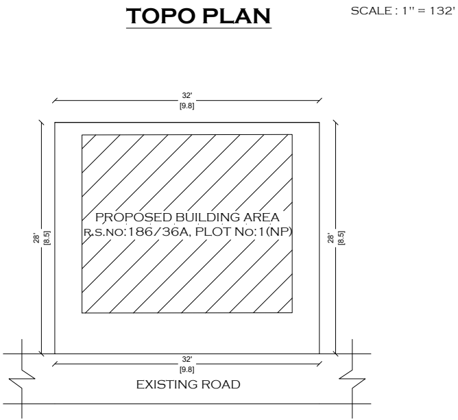
EXTENT DETAILS
