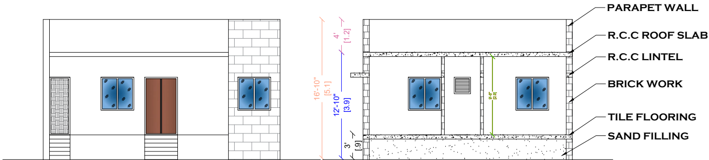
SECTION ON 'A-A'
