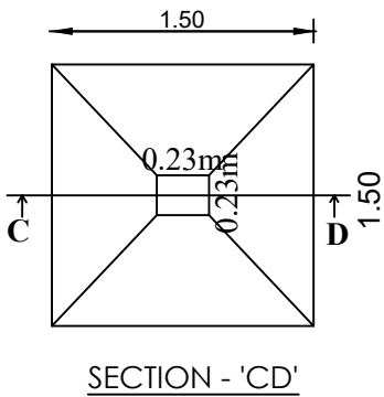
SECTION - 'CD'
