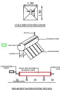
SOLAR HOT WATER SYSTEM DETAILS
