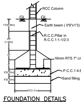
FOUNDATION DETAILS
