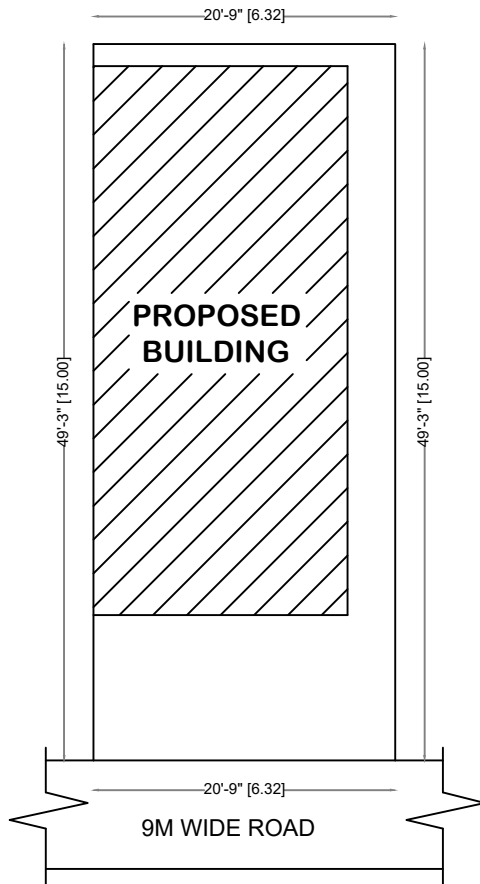
SITE PLAN
