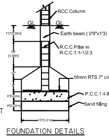
FOUNDATION DETAILS
