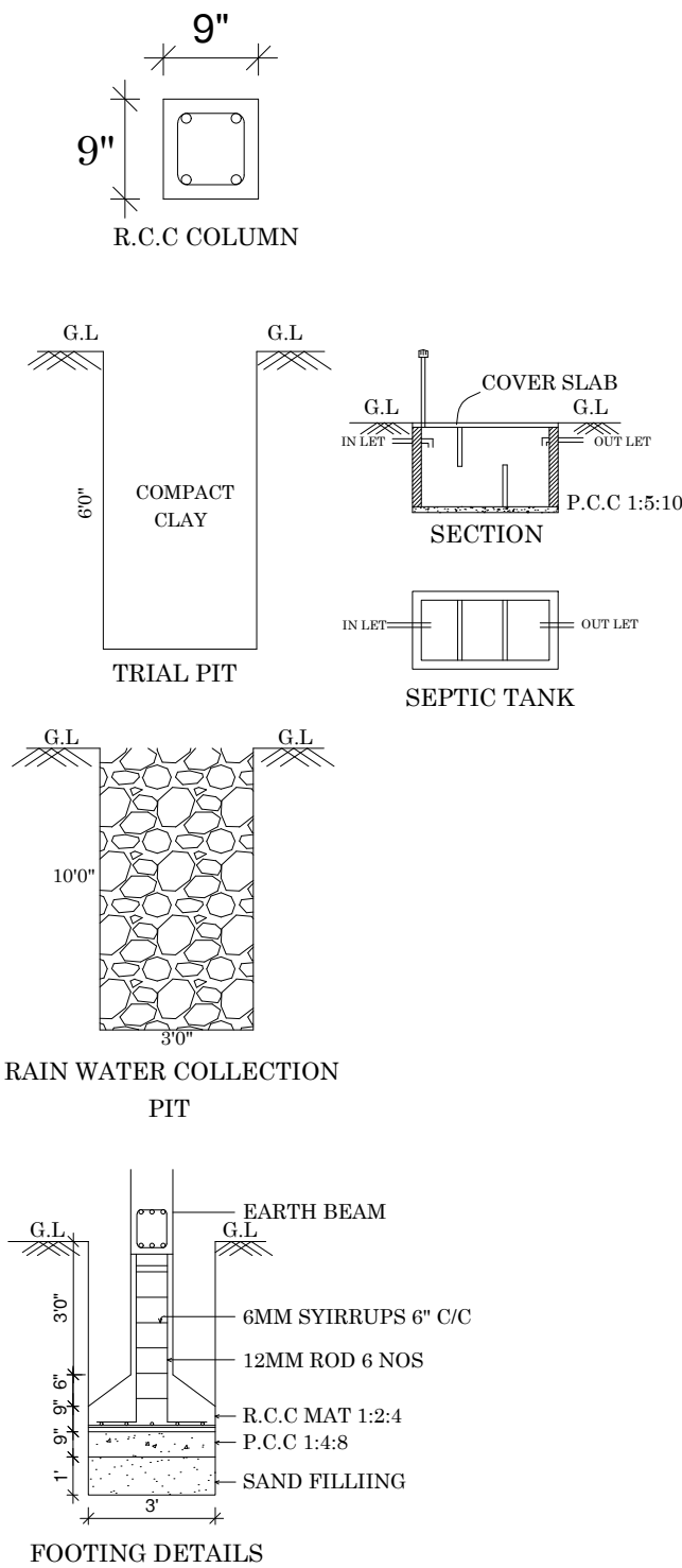
FOOTING DETAILS
