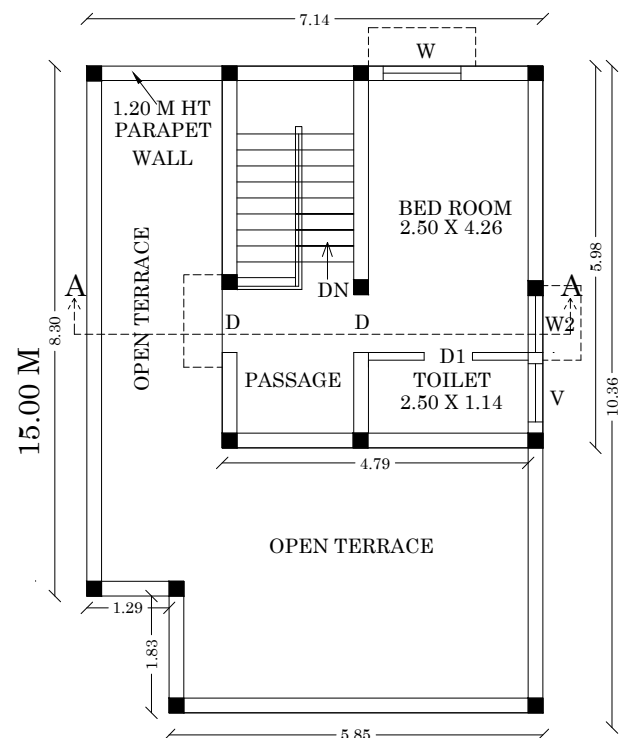
FRIST FLOOR PLAN
