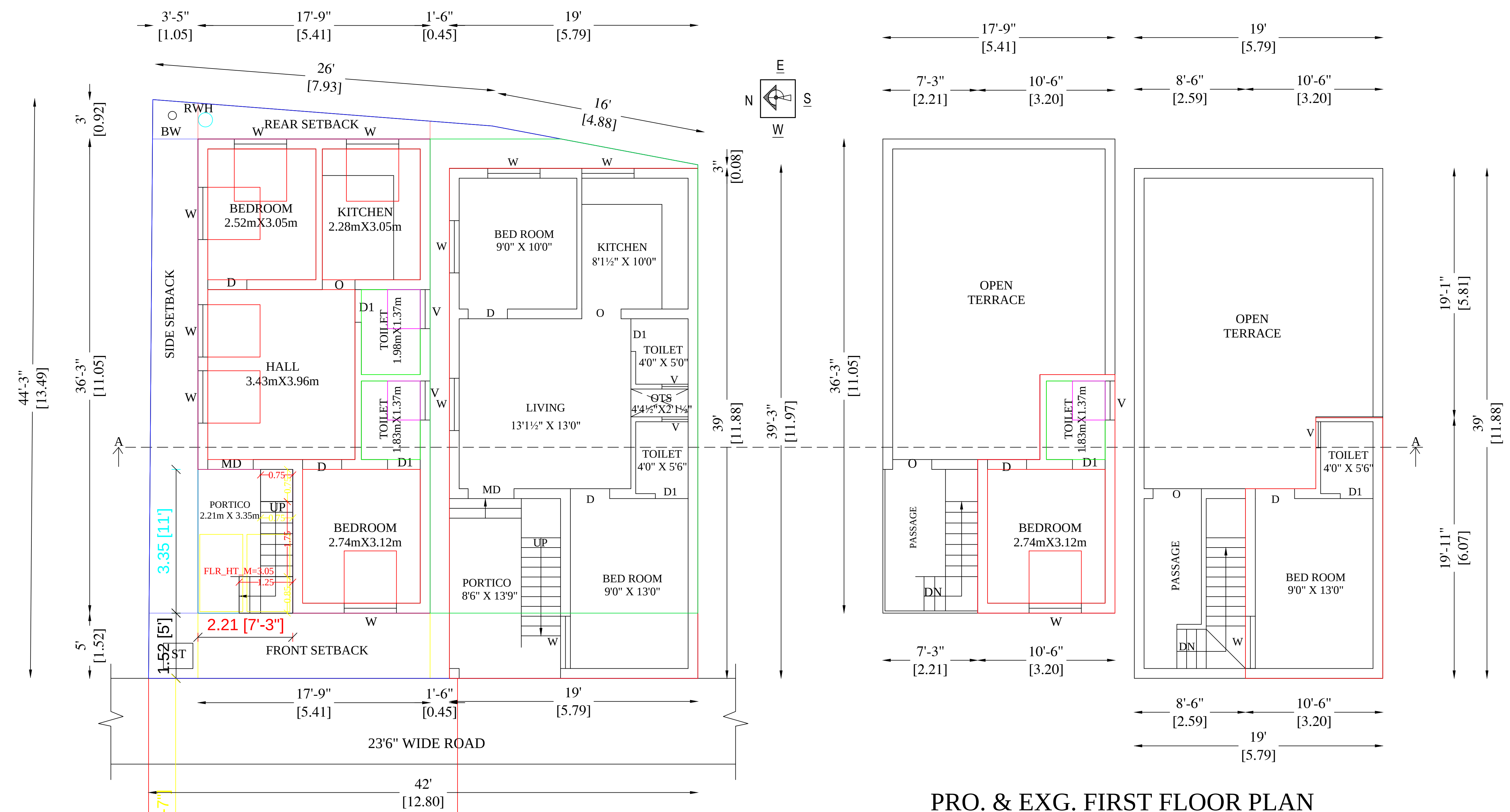
PRO. & EXG. FIRST FLOOR PLAN
