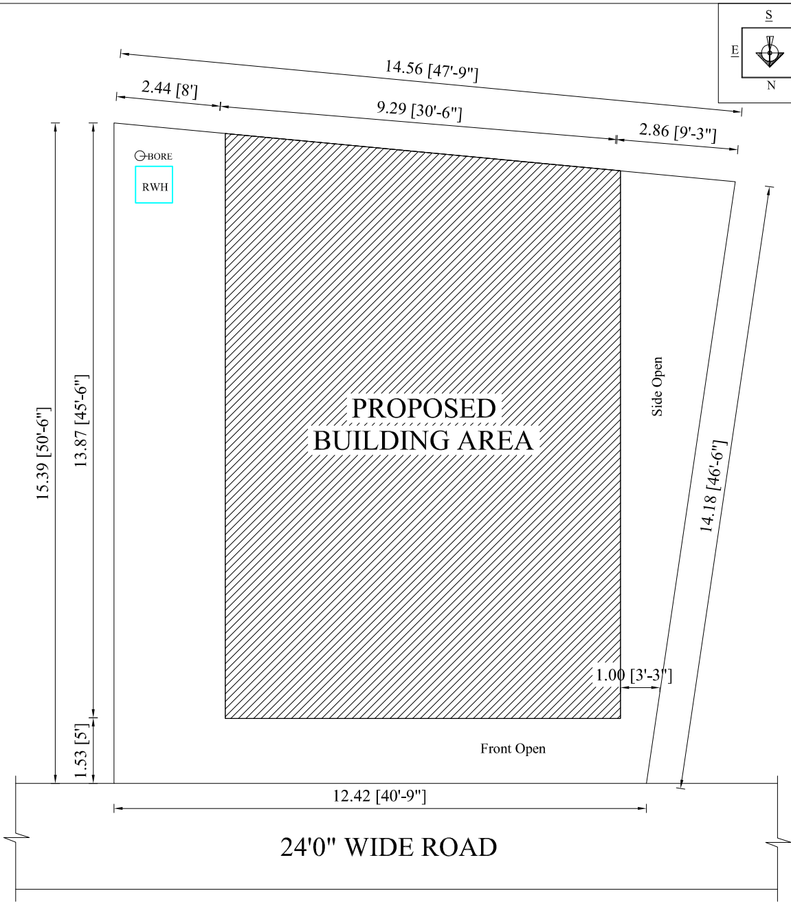
SITE PLAN
