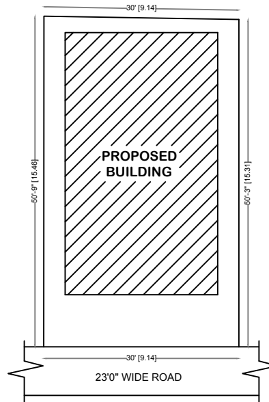
SITE PLAN
