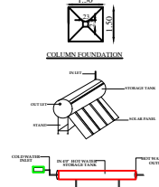
SOLAR HOT WATER SYSTEM DETAILS
