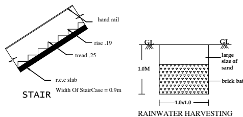
RAINWATER HARVESTING
