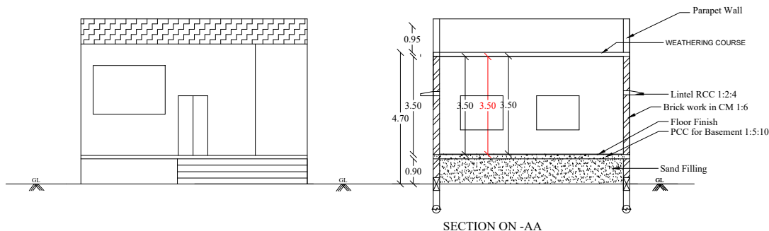
FRONT ELEVATION
