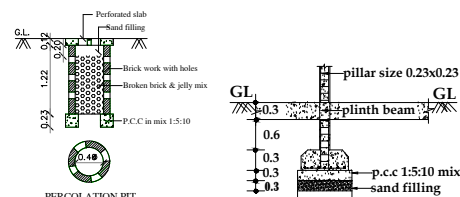
PERCOLATION PIT
